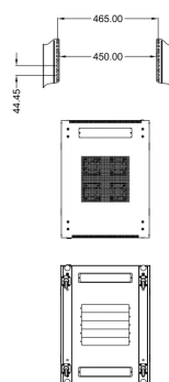
Top / bottom mounting views (dimensions in mm)
