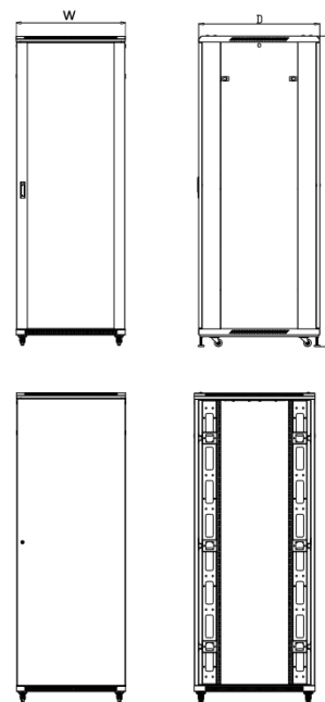
Front / side / rear / side (no panel) views
